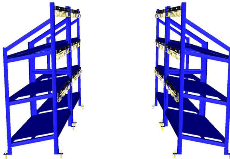
ISO View – 3X6 PTL Setup
